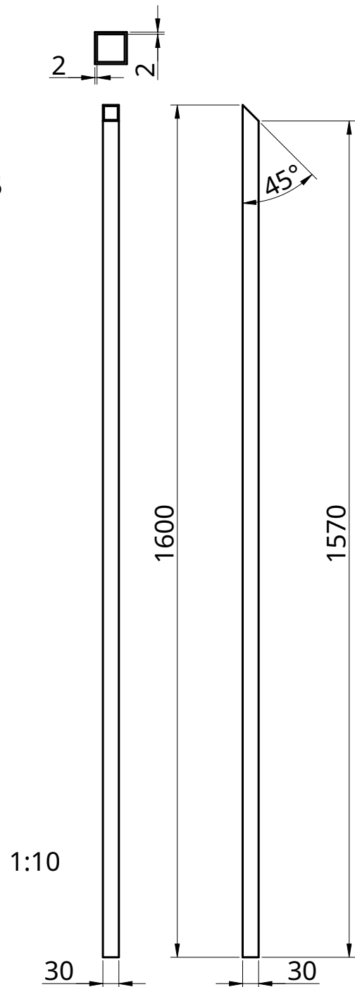
POTEAU 1:5
